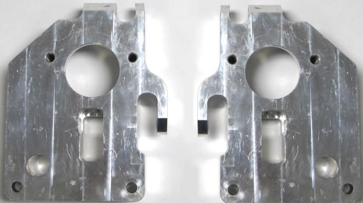
Rear Left Backing Plate PGLC-BP-RZR1-RL (1ea)
